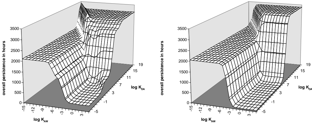
Fig. 5A Dependence of overall persistence on physical chemical properties as expressed by log K OA and log K AW . Assumptions: Equal fraction of emissions into air, water and soil. Half-lives 48 h in air, 1460 h in water and 4380 in soil. Level III on the left, level II on the right.
